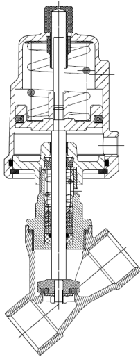
Diagram of Normally Closed Valve
