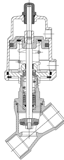
Diagram of Normally Open Valve
